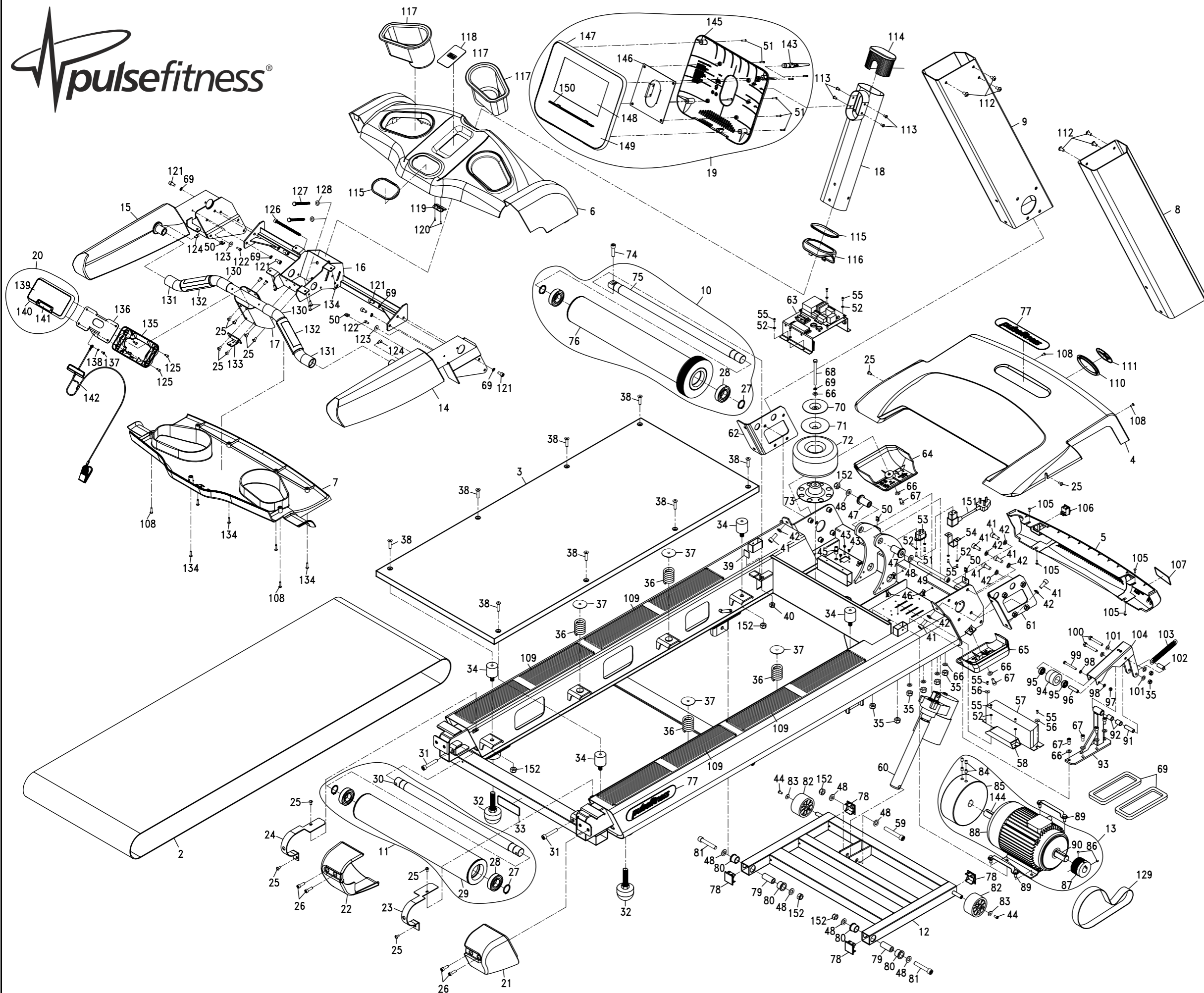
260G Exploded Drawing
